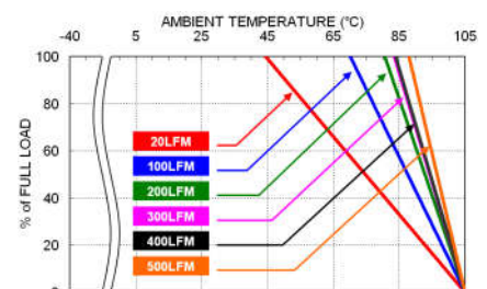
QAE100-24S05W Derating Curve With 0.5" Height Heat-sink
