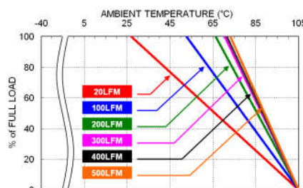
QAE100-24S05W Derating Curve With 0.24" Height Heat-sink
